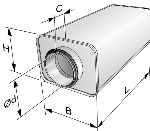
Figure 2. CLA-A – Dimension print
