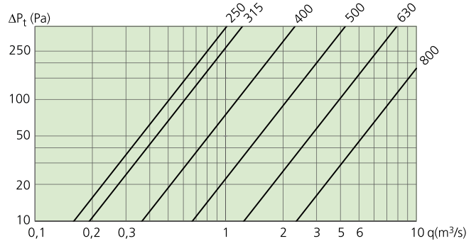
Diagram 2. Pressure drop – Airflow, CLA-B
