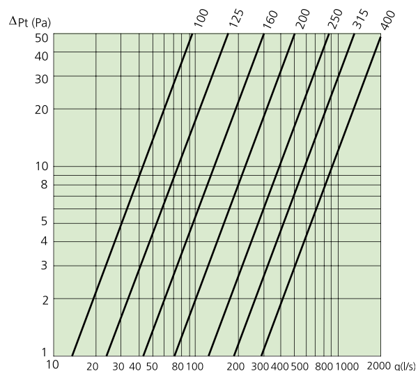
Diagram 1. Airflow – pressure drop, SORDO-A, C
