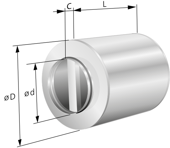
Figure 4. SORDO-B – Dimension print
