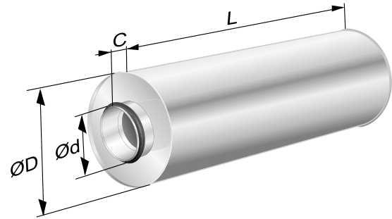
Figure 2. SORDO-A – Dimension print
