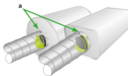
Figure 1. For reasons of safety, connect the connection duct to the raised sheet-metal edge that is fastened inside the connection spigot using screws or pop rivets (a).
