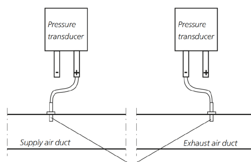
Fig.4: Pressure sensor location
