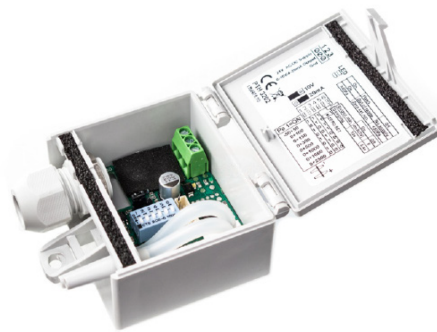
Fig.1: PRESSURE SENSOR 0...10V CID521249
